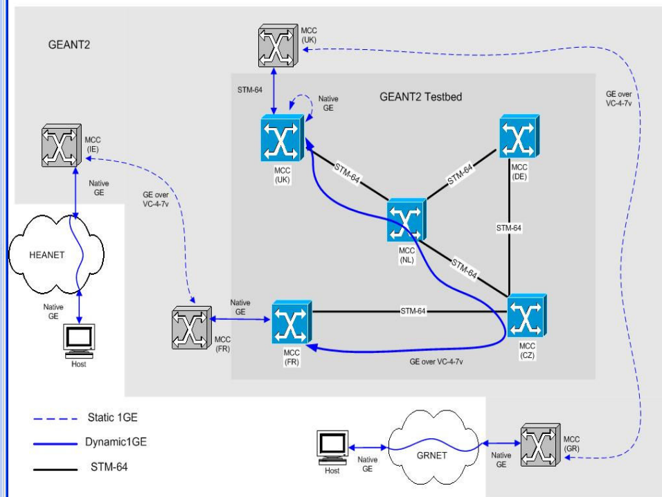
AutoBAHN demonstration circuit
